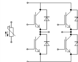
H-bridge
