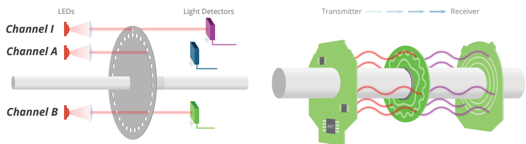
Figure 1: Unlike an optical encoder that relies on line of sight optics, the AMT utilizes an electromagnetic field to transmit signals, eliminating vulnerabilities to environmental contaminants such as dust, dirt and oil
