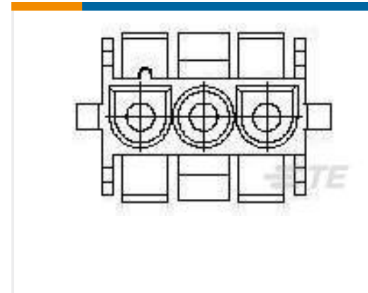
TE Part #794900-1 03P UMNL HI TEMP CAP HSG
