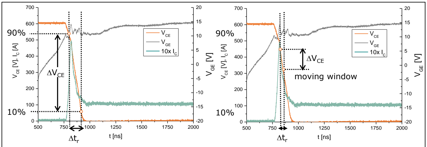
Figure 6 Example of turn-on switching curves for a) dv/dt_{10-90} definition b) dv/dt_{max} definition for FS100R12W2T7 at 10% I_{Cnom} , T_{vj} = 25^\circ C
